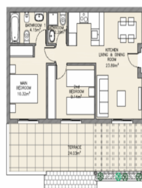
MAIN FLOOR
